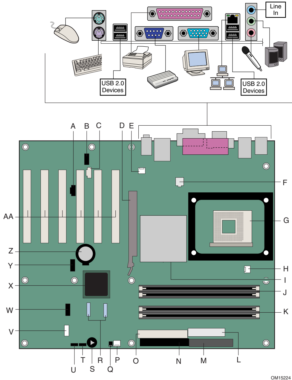
Figure 1. Desktop Board D865GBF Components
